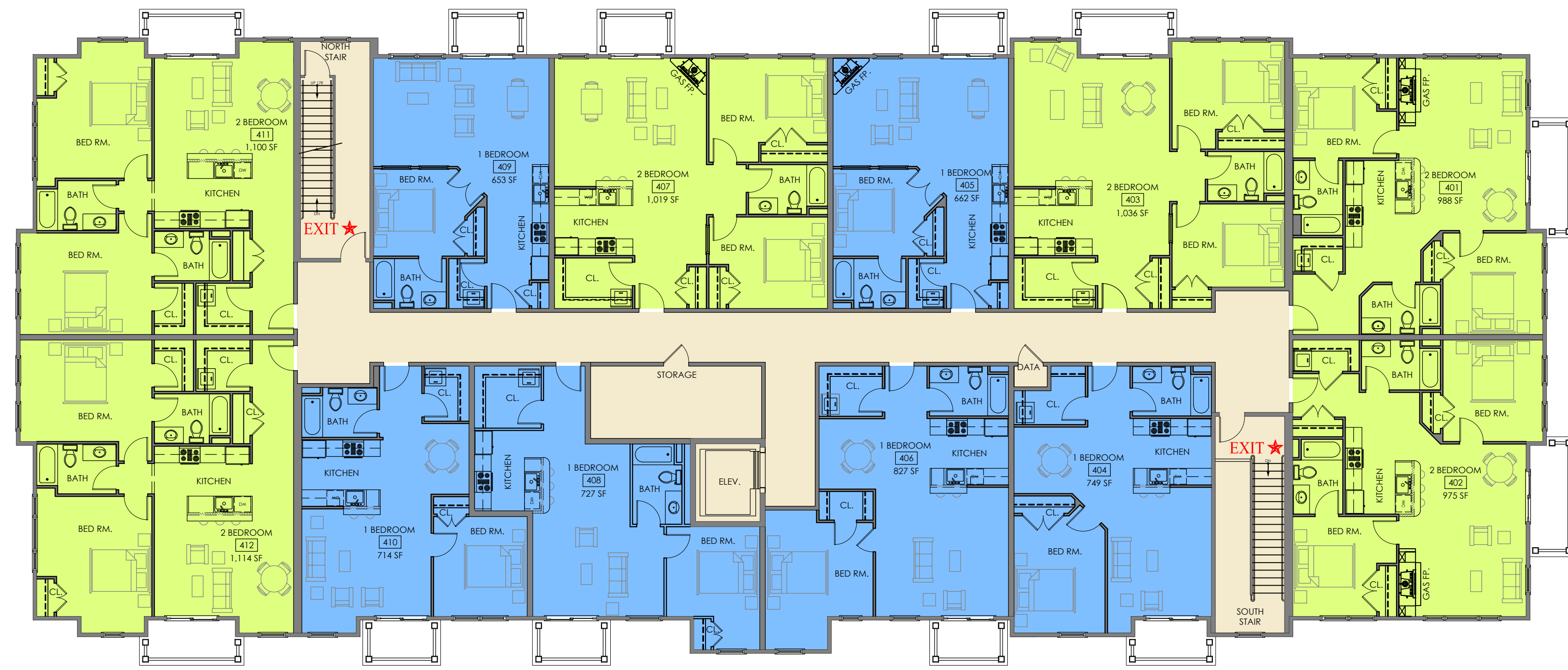
FOURTH FLOOR PLAN
